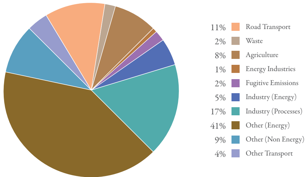
Figure 2 The emission factors (EFs) of POP from the different sources (2)
